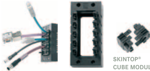
SKINTOP® CUBE
