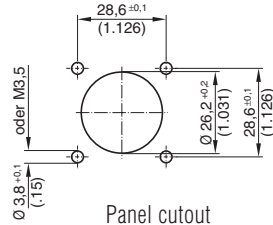
Panel cutout
