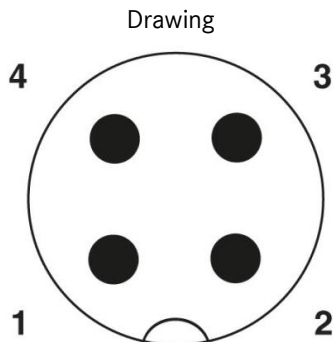
Pin assignment M12-plug Y, 4-pol, A-coding
