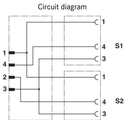
Pin assignment between M12-plug Y and M8-jack
