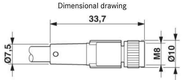
Jack M8 x 1, straight
