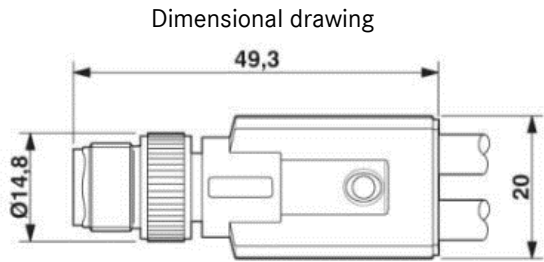
Plug Y, M12 x 1, straight
