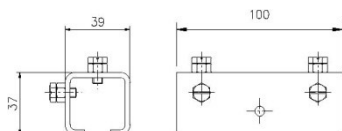
Track coupler Material: Galvanized steel Weight, kg: 0,28 Article No.: 62200423
