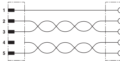
S/A DeviceNet/CANopen cable, M12 connector on M12 socket
