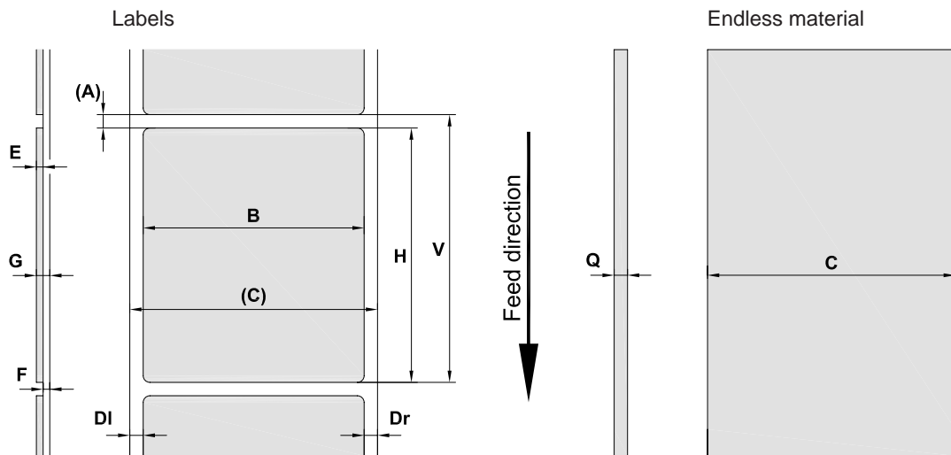
Fig. 14 Label / endless material dimensions
