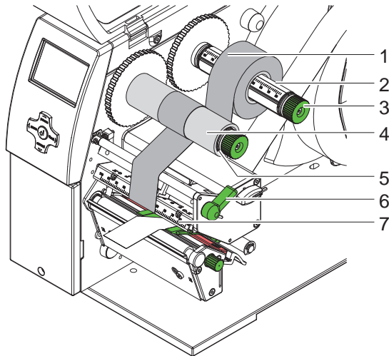
Fig. 10 Loading transfer ribbon
