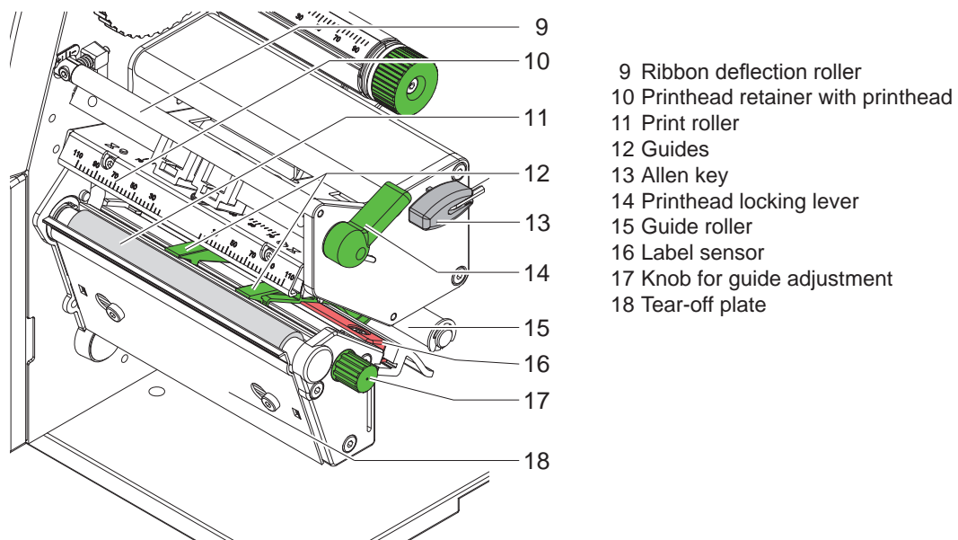
Fig. 2 Print mechanics
