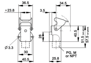
EPIC® HA 3/4 Surface Mount Base; palanca sencilla
