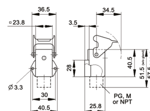
EPIC® HA 3/4 Surface Mount Base; palanca sencilla
