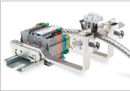
Spring shield clamping saddles on a horizontal bussbar with metal T-connector
