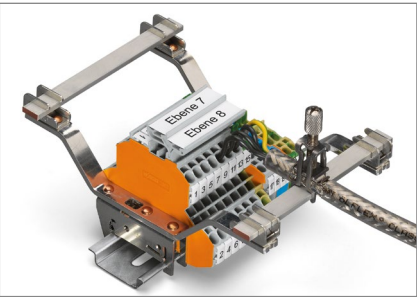
Screw shield clamping saddles on a horizontal bussbar with both-side, angled metal carriers
