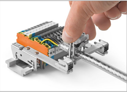
Fitting a spring shield clamping saddles to a bussbar with single, straight metal carrier.
