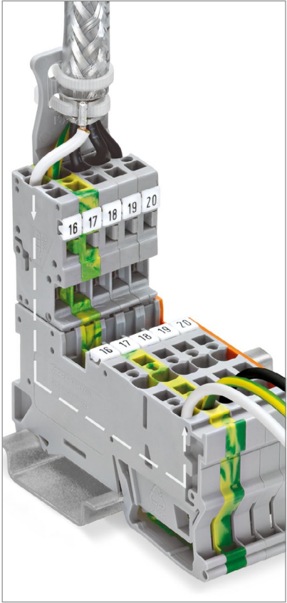
Shield termination connected to an X-COM® modul
