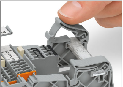
Fitting a busbar to an insulated carrier 14 15 16 30
