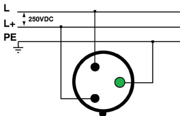
250VDC; 2+PE, 3-wire, 3h
