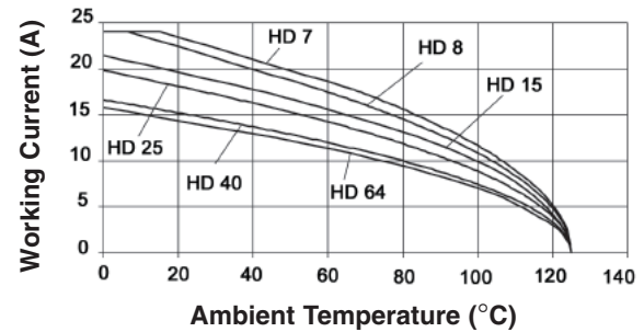
HD CRIMP MACHINE: 1.5 mm 2 (16 AWG)
