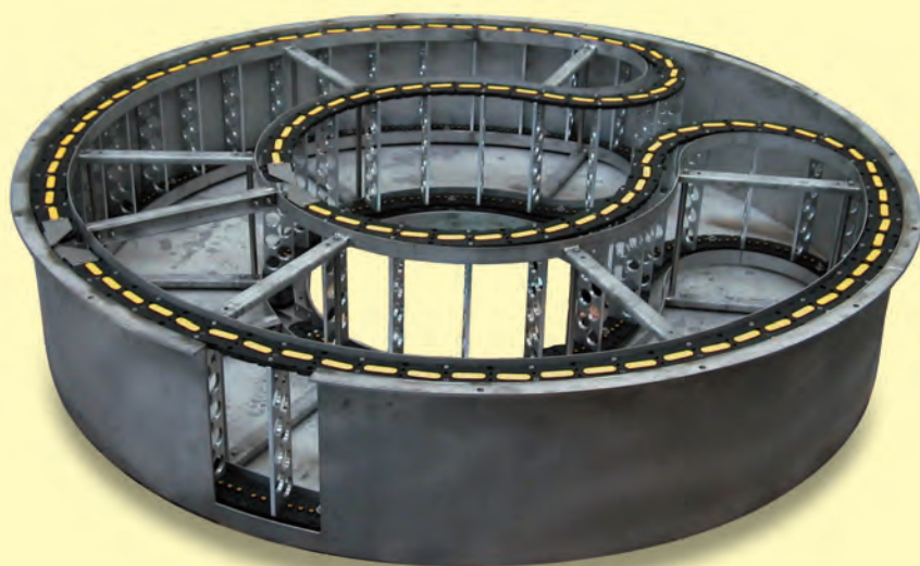
Application with 2 chains. Rotation 370^\circ
