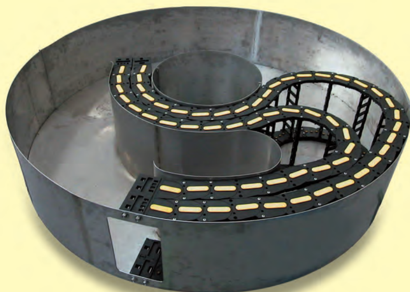
Application with 2 superimposed chains. Rotation 180^\circ
