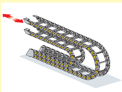
Superimposed chains.
