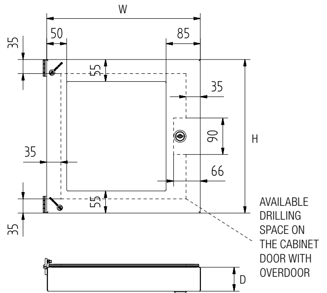
VERSION WITH 1 CLOSING POINT
