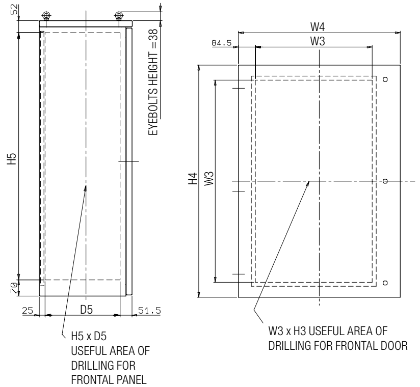
FRONT DOOR DETAIL CABINETS
