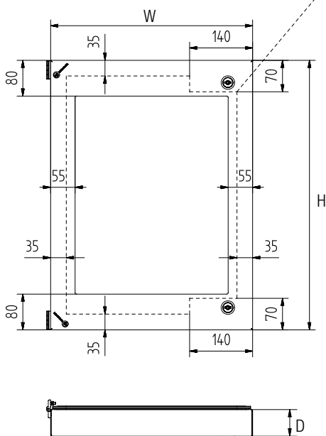
AVAILABLE DRILLING SPACE ON THE CABINET DOOR WITH OVERDOOR
