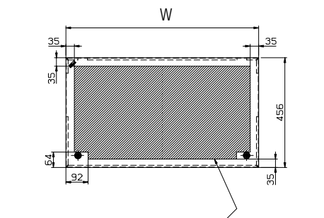
AVAILABLE DRILLING SPACE ON THE UPPER DOOR
