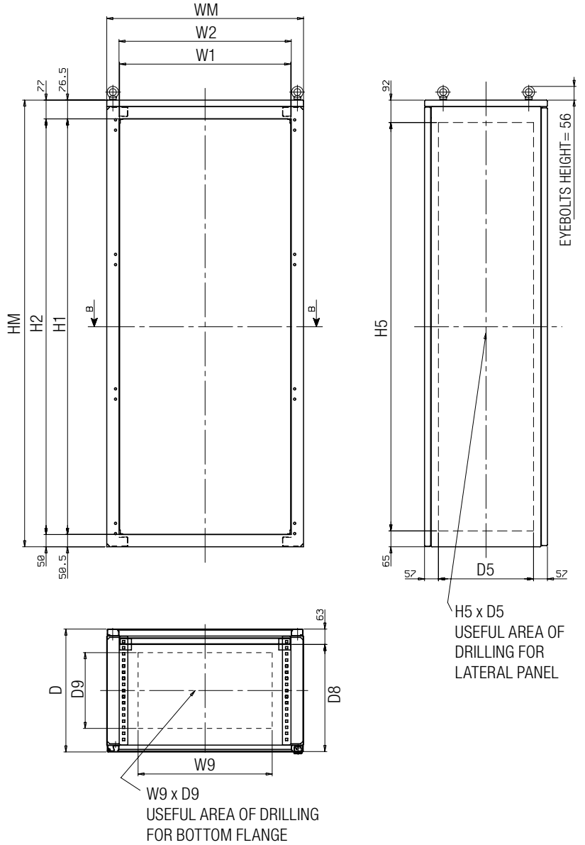
FRONT VIEW WITHOUT DOOR
