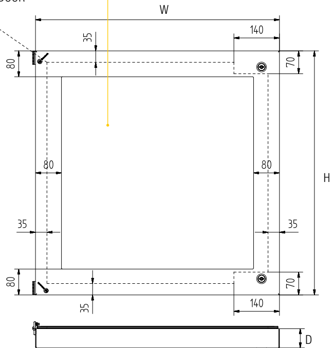
1. MODELS FRONT VIEW ***
