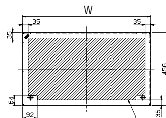
AVAILABLE DRILLING SPACE UPPER DOOR
