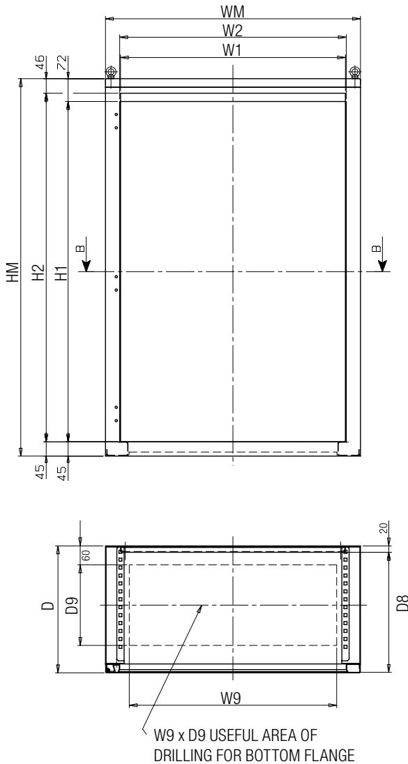
FRONT VIEW WITHOUT DOOR
