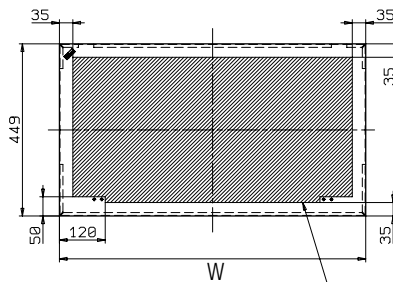
AVAILABLE DRILLING SPACE ON THE UPPER DOOR
