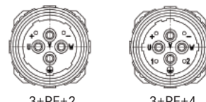
Style A6: View from contact side
