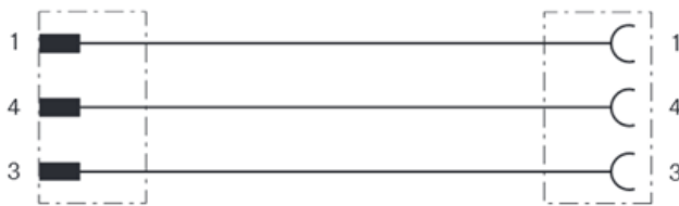
Pin assignment between M8-plug and M8-jack
