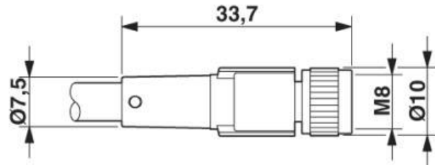
Jack M8 x 1, straight
