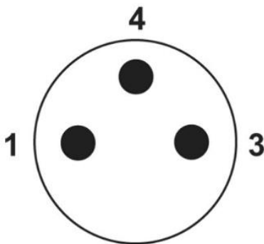
Pin assignment M8-plug, 3-pol, A-coded
