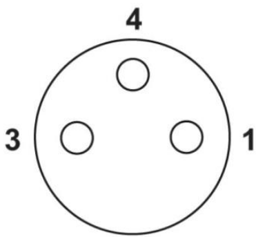
Pin assignment M8-jack, 3-pol, A-coded
