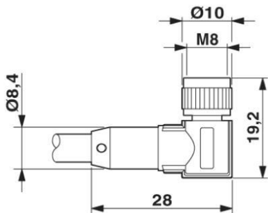
Jack M8 x 1, angled, with LED
