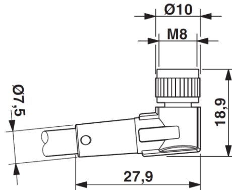
Jack M8 x 1, angled
