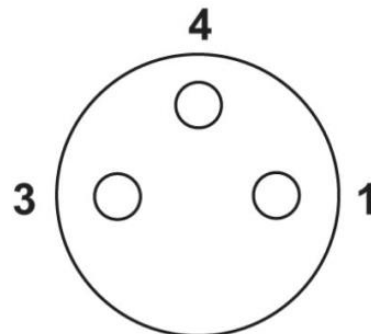
Pin assignment M8-jack, 3-pol, A-coding
