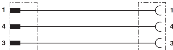
Pin assignment between M12-plug and M8-jack
