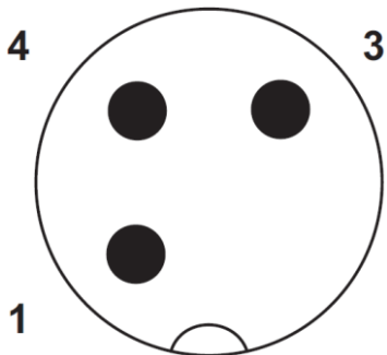
Pin assignment M12-plug, 3-pol, A-coding
