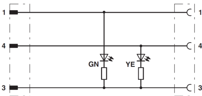
Pin assignment between M8-plug and M12-jack
