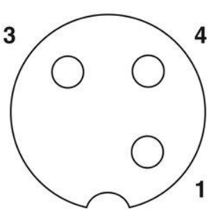
Pin assignment M12-jack, 3-pol, A-coding
