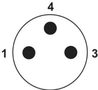
Pin assignment M8-plug, 3-pol, A-coding
