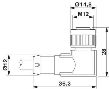
Jack M12 x 1, angled, with LED
