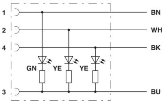
Circuit diagram
