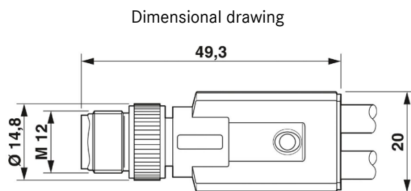
Plug Y, M12 x 1, straight
