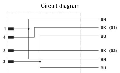
Pin assignment M12-plug Y
