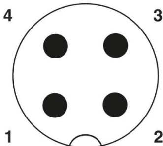
Pin assignment M12-plug Y, 4-pol, A-coding
