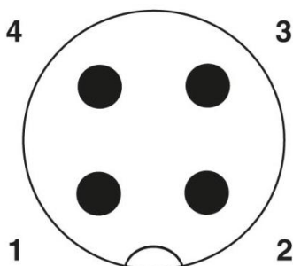
Pin assignment M12-plug Y, 4-pol, A-coding
