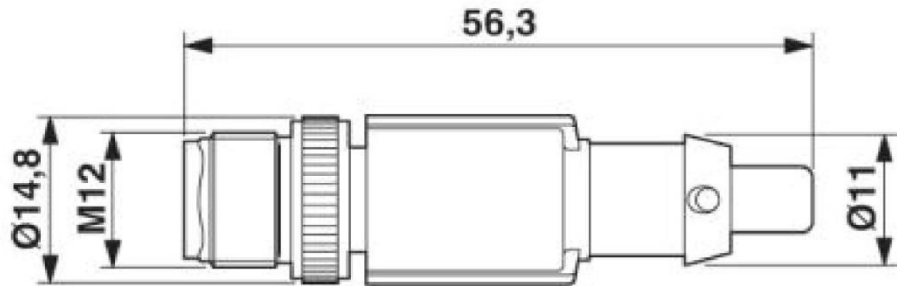
Plug M12x1, straight, shielded
