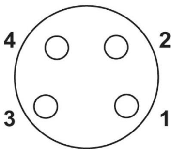
Pin assignment M8-jack, 4-pol, A-coding
