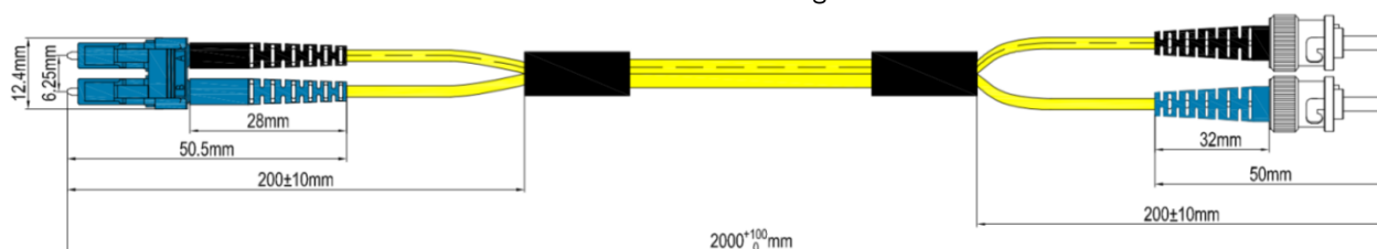
Dimensional drawing
