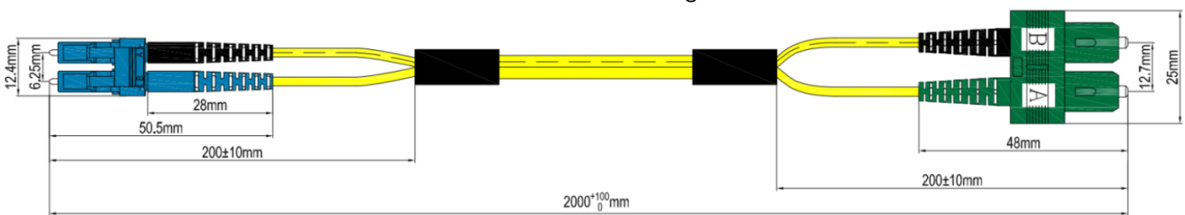
Dimensional drawing
