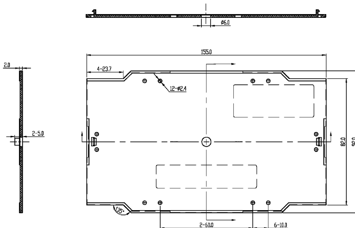
Dimensional drawing
