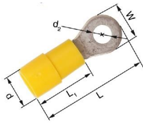
Ring cable lugs
